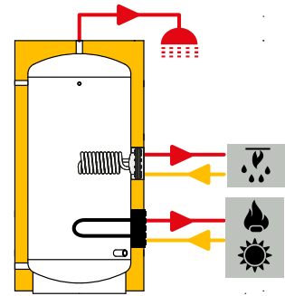
Connection legend
