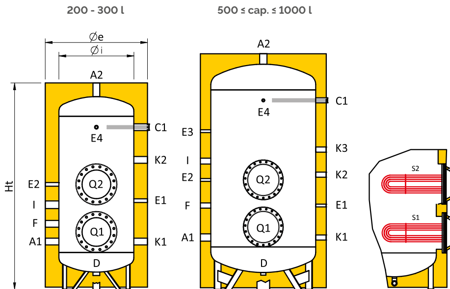
Connection table
