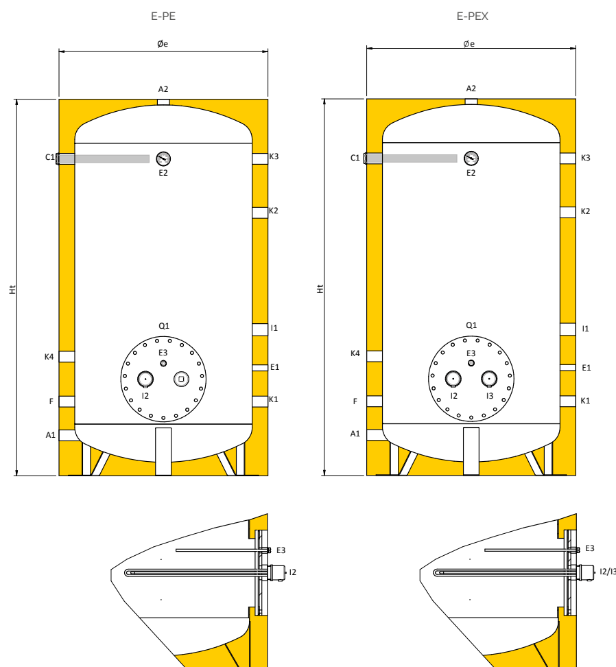
Connection legend
